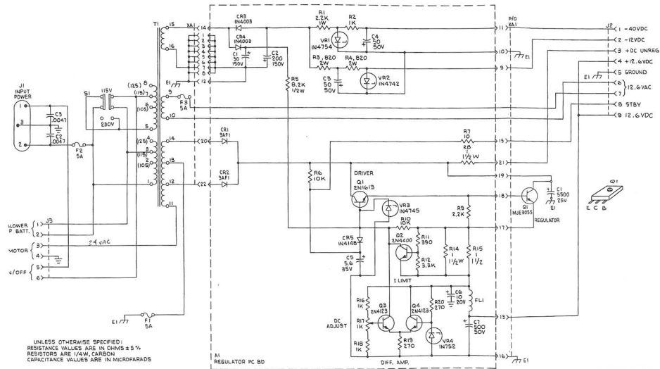
Figure 10 - 2. Power Supply Module A5, Schematic Diagram
