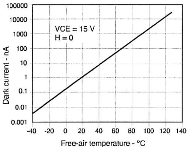
Fig. 3 Dark Current vs Temperature
