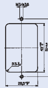
Panel cut-out
